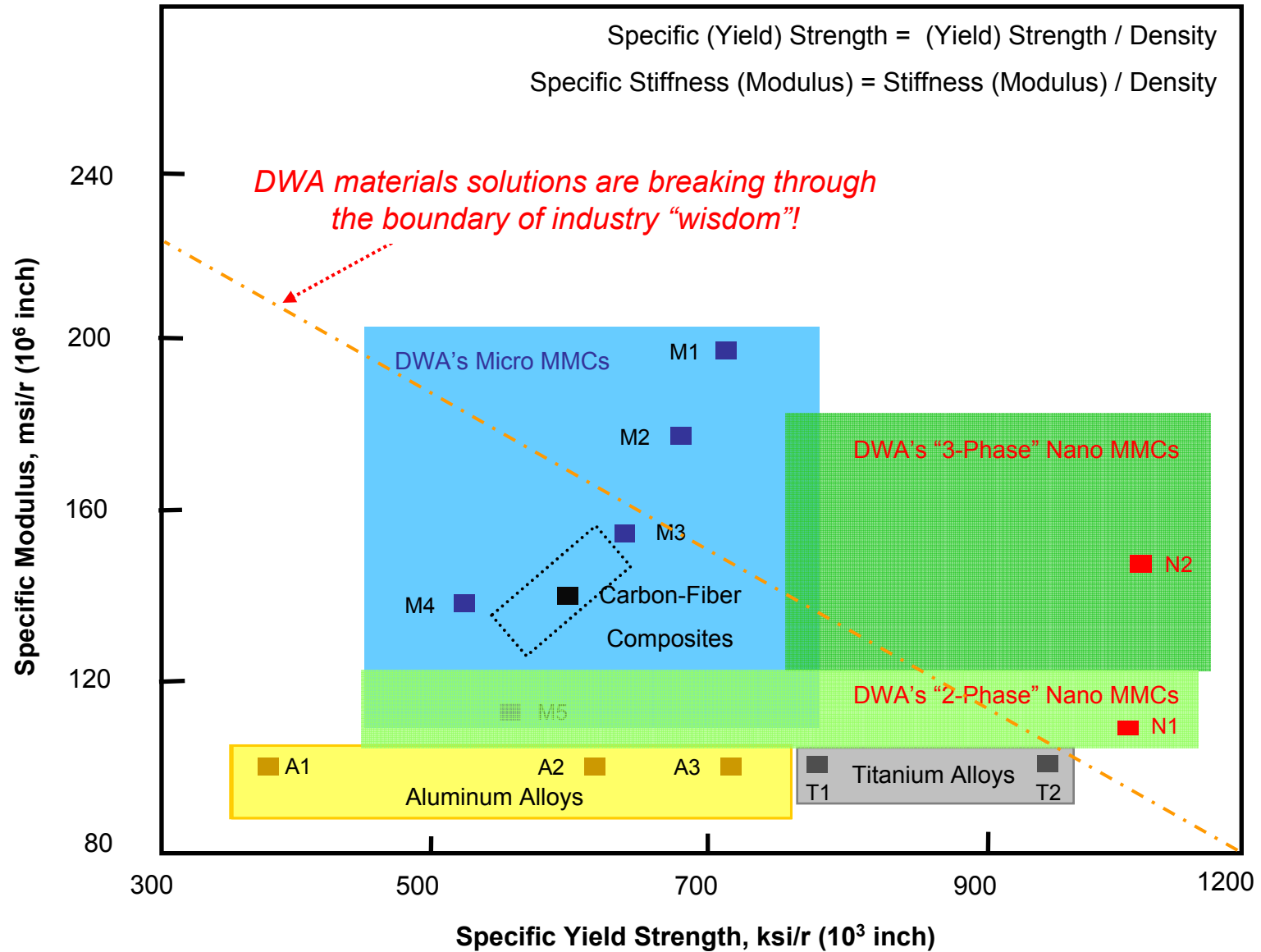
Figure 1. Specific Property Comparison of DWA's Micro & Nano MMCs, Aluminum Alloys, Titanium Alloys and Carbon-fiber Composites
